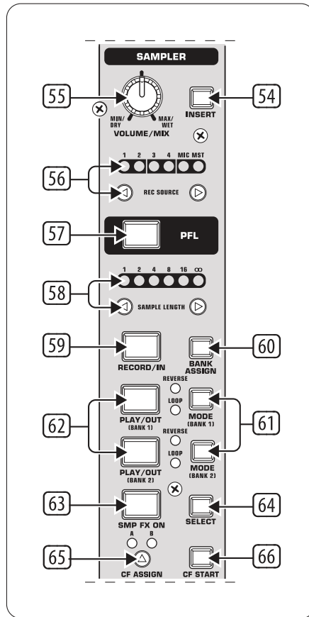
Figure10: Sampler section
