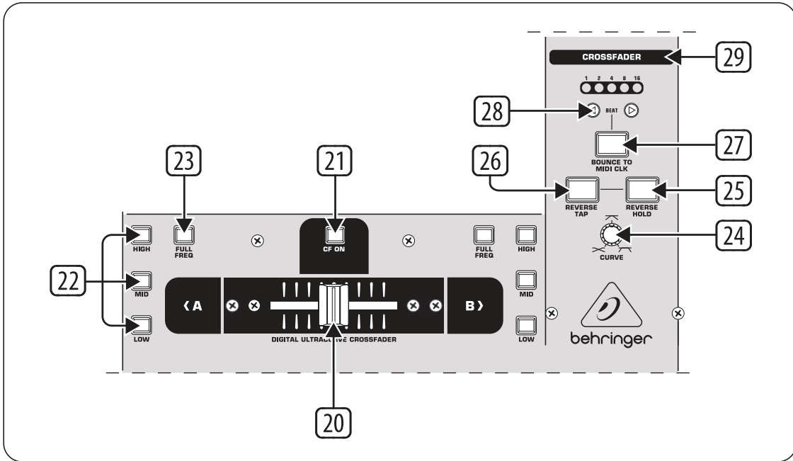
Figure9: Crossfader section
